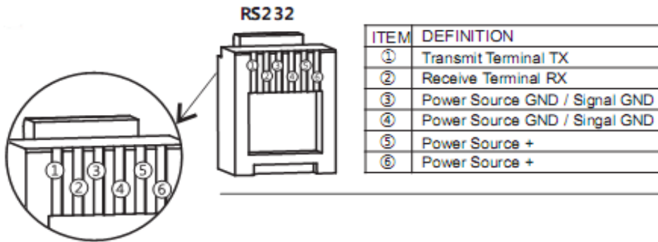
Figure 1-1 Solar Charge Controller Appearance and Interface
